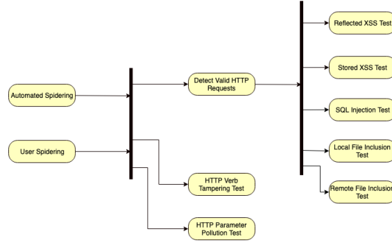
Fig. 2. Hacking Tasks Tree Example for Web Applications
