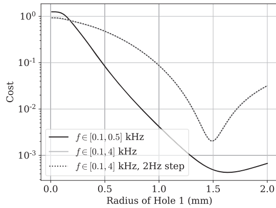
Figure 7. Cost evolution with respect to the radius of Hole 1 on the fingering “xxxx”, with three frequency ranges: [0.1, 0.5] kHz and [0.1, 4] kHz with a 100 Hz step, and [0.1, 4] kHz with a 2 Hz step.
