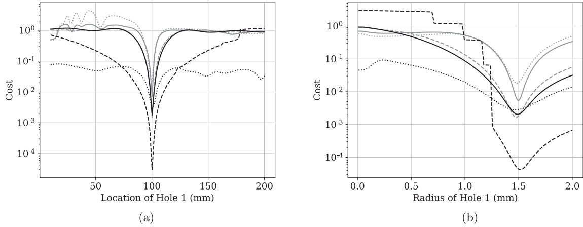
Figure 4. Costs evolution for different observables computed for frequencies in [0.1, 4] kHz with a 2 Hz step, for the fingering “xxxx” with respect to: (a) the location and, (b) the radius of the first hole. The observables are: the complex value (solid lines), the modulus (dotted lines) and the phase (dashed lines) of the impedance (gray) and the reflection coefficient (black).
