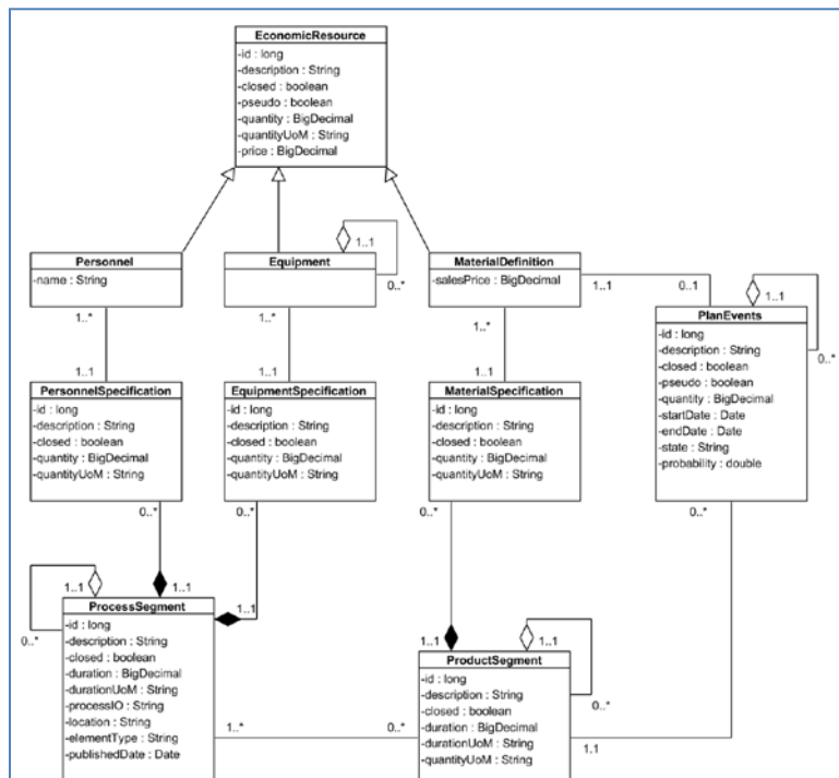
Figure 7: ERP-CONTROL: Stochastic production planning – Inclusion of Plan Events
