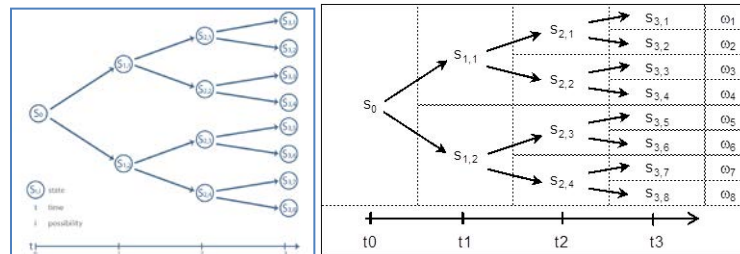
Figure 2: Binary uncertainty sample space – Possible occurrences of the worlds over time
