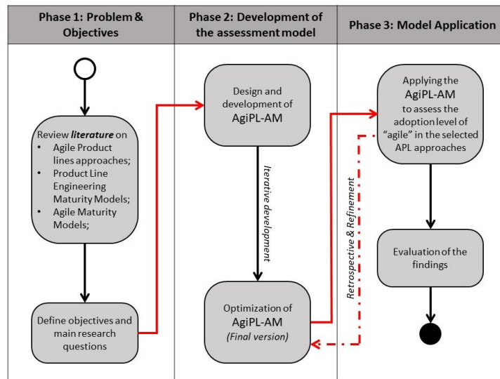
Fig. 1. Research procedure
