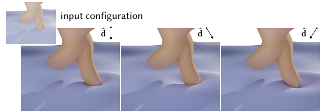
Fig. 21. Control over the mapping direction \hat{d} . Left: using the automatic direction. Middle and Right: modifying the mapping direction permits to mimic friction effects. [ k_{\text{finger}} = 0.9 , \phi_{\text{ground}} = 50 , \phi_{\text{finger}} = 20 , \tau = 0 ]
