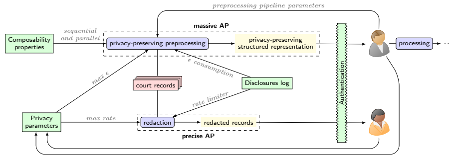
Fig. 3. Multimodal publication architecture
