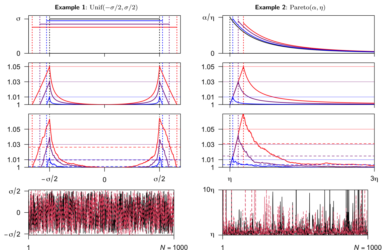
FIG 1. Illustrations with M = 4 chains, N = 1000 iterations each. Colors blue, violet and red resp. correspond to choices of ‘diverging’ distributions F_M such that our scalar diagnostic R_\infty matches with 1.01, 1.03 and 1.05. Top row: density of distributions F_m used, uniform (left) and Pareto (right). Colors for ‘diverging’ F_M and black for others. Second row: population (theoretical) version R(x) of our index. Third row: empirical version \hat{R}(x) of our index on simulated data; discussed rank- \hat{R} shown as colored dashed lines. Bottom row: traceplots of one ‘converging’ chain ( m = 1 , black) and the ‘diverging’ chain ( m = M , red case, R_\infty = 1.05 ).
