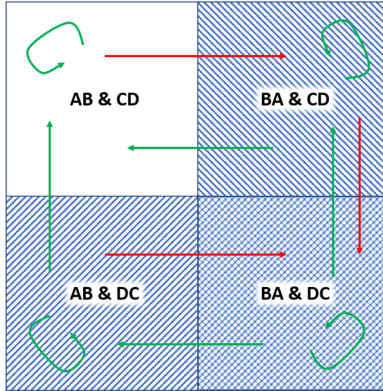
Fig. 2: Moves prohibited in red and allowed in green with GP = \{AB, CD\} .
