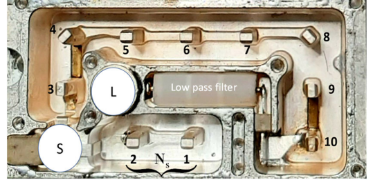
Fig. 6. Fabricated structure of the path filter. The resonators are the numbered square cylinders (1 and 2 are those realizing the transmission zeros).
