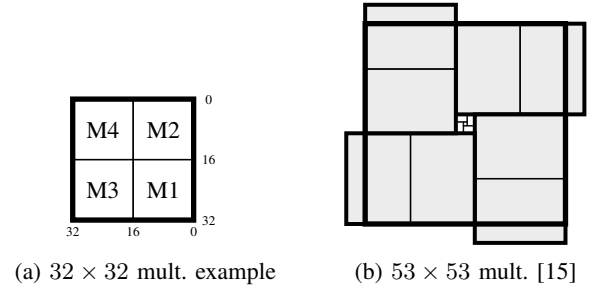
Fig. 1: Tilings for realizing different multipliers
