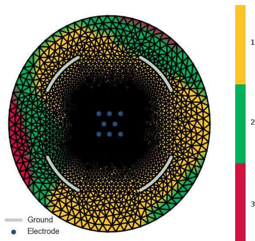
Fig 13. Section 4.2: Finite element mesh representing one well, including 8 electrodes of the 96-well MEA device from Axion Biosystems.
