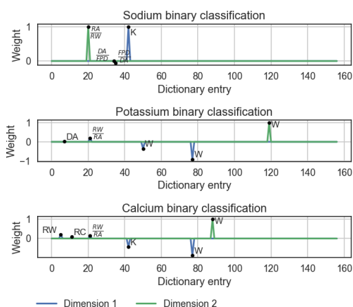
Fig 14. Weights obtained by the optimised classification algorithm. See Section 4.2, Binary classification part.
