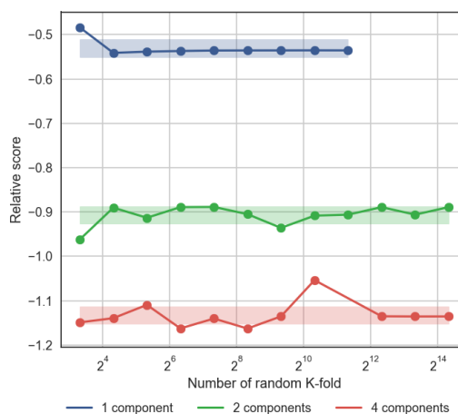
Fig 22. Impact of the number of repeated k-fold on the cost function in the torsadogenicity classification with the \Delta_{min} = 0.02 range.
