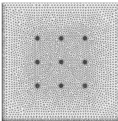
Fig 9. Section 4.1: Finite element mesh representing one well including 9 electrodes of the 6-well MEA device from Multichannel Systems.
