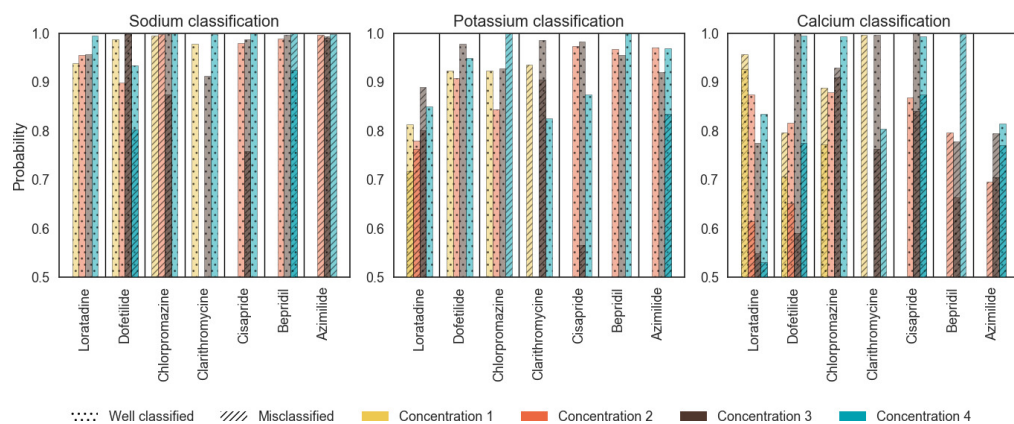
Fig 17. Section 4.2, Binary classification part: Experimental data classification in binary case for each concentration (some concentrations were not used due to the quiescence or noisy signal observation). For each concentration, the LDA classifier returns the average probability for well classified (dotted bars) and misclassified (hatched bars) compounds.
