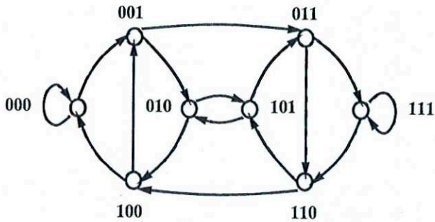
Fig. 1. Example of a de Bruijn digraph B(2, 3) .
