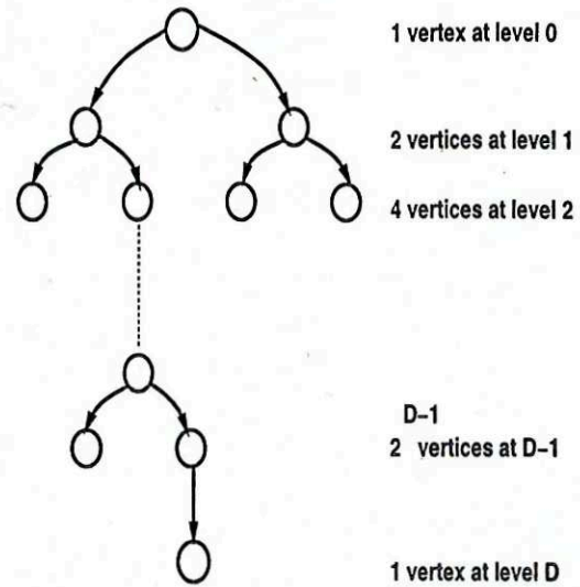
Fig. 2. Shortest path tree with the minimal weight.
