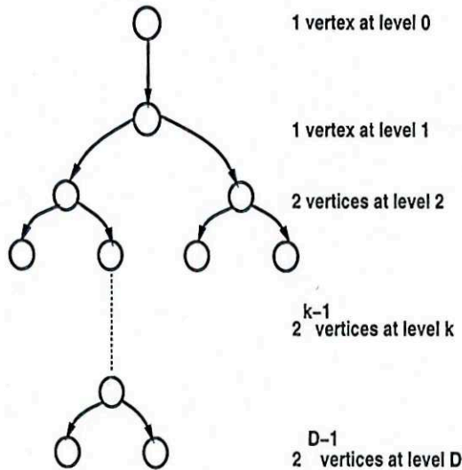
Fig. 3. Shortest path tree with the maximal weight.
