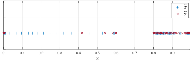
Figure 9: Quadrature points delivered by the ECSW method to approximate the volume (blue) and surface (red) integrals for M = 8 .
