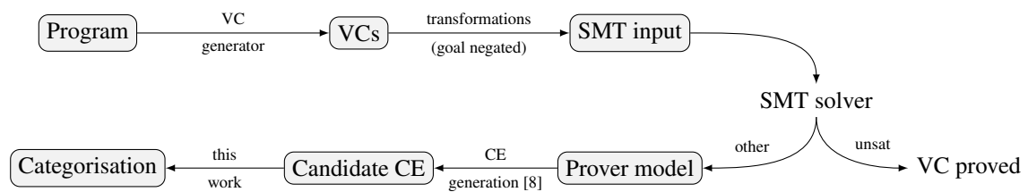
Figure 20: Pipeline of the Why3 counterexample (CE) generation and categorisation
