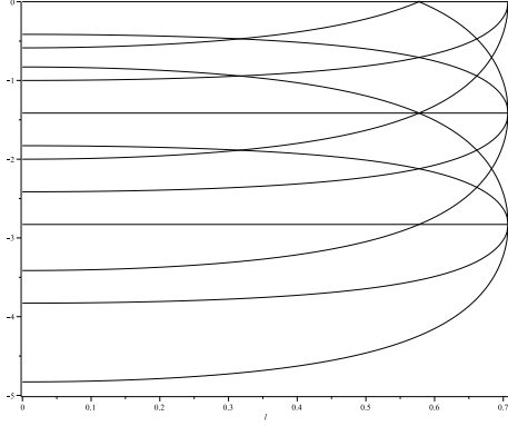
Fig. 3. The sum of exponents in function of \ell for all possible choices of \epsilon, \kappa . When one of these curves intersects a non positive integer ordinate, equation (16) for the corresponding \ell has a resonance between its exponents.
