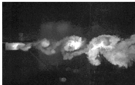
Mixing layer downstream a thick plate
