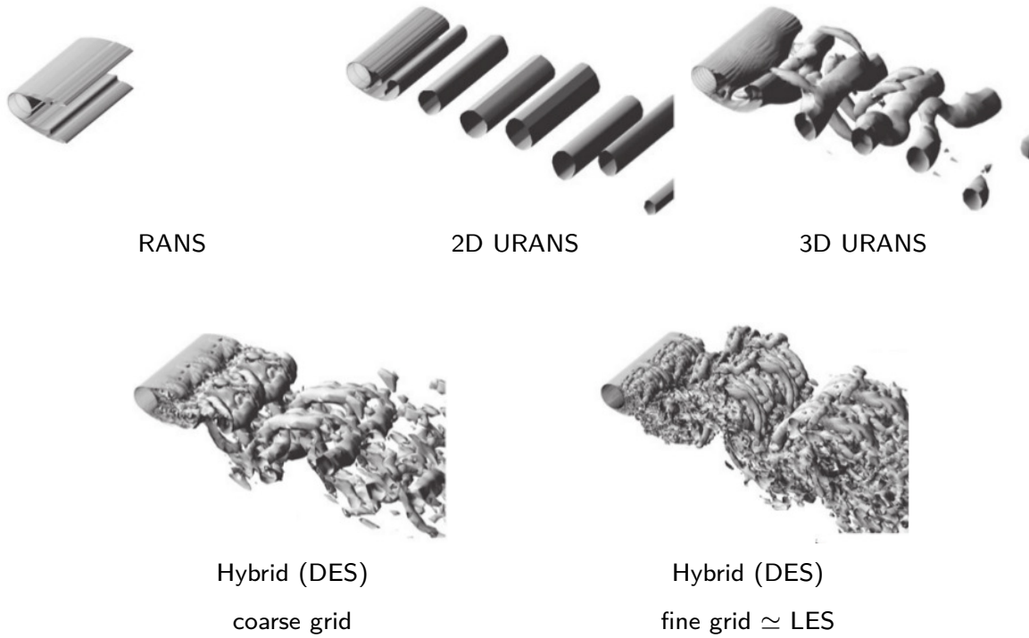
From Spalart (2009), Re = 50000 .
