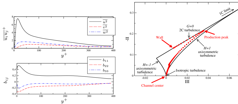
DNS data of Kim et al. (1999) in a channel flow at Re_\tau = 395
