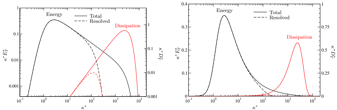
Energy (axis on the left) and dissipation (axis of the right) spectra in log-log scale (left) and log-lin (right). Quantities are made non-dimensional using k and \varepsilon .
