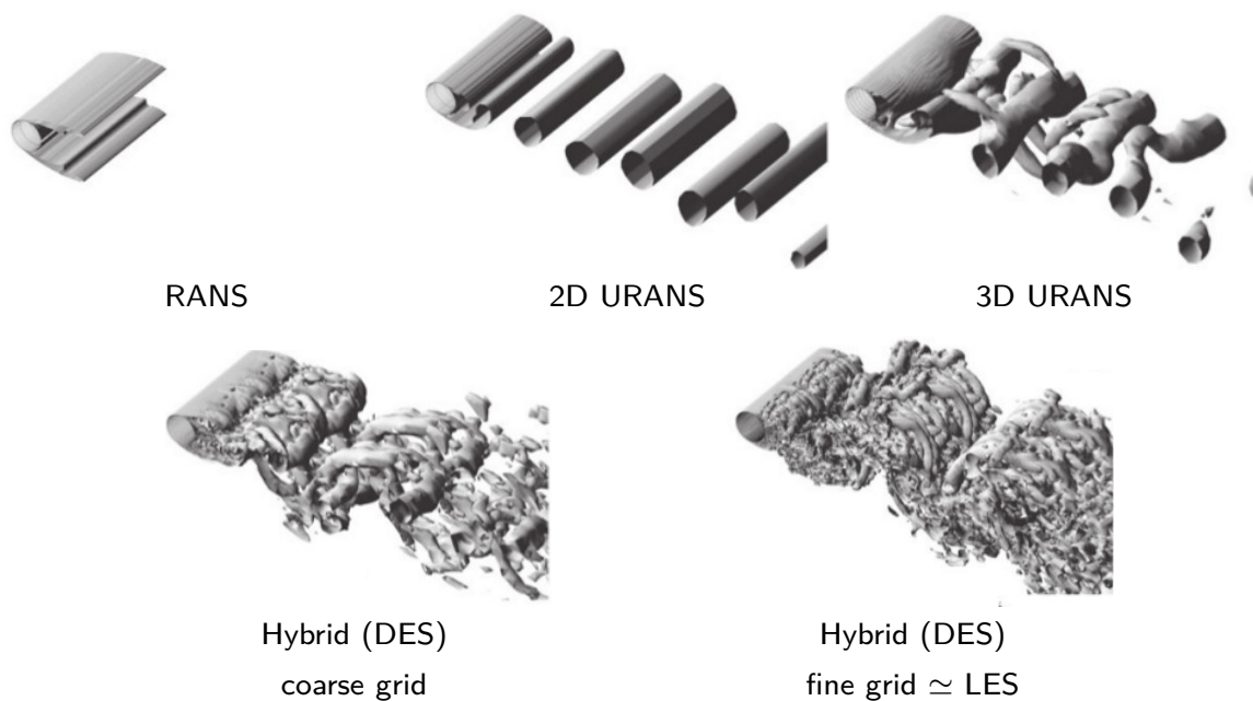
From Spalart (2009), Re = 50000 .
