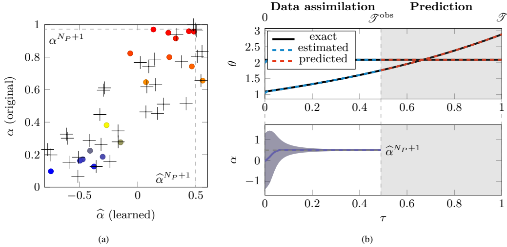
FIGURE 6 Test Case 2: (a) original parameters \alpha^i plotted against the corresponding learned parameters \hat{\alpha}^i and (b) evolution of \theta^{N_P+1}(\tau) , of \hat{\theta}^{N_P+1}(\tau) and of the estimation of \hat{\alpha}^{N_P+1} . See caption of Fig. 5 for the notation.
