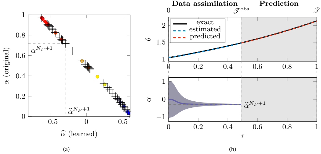
FIGURE 5 Test Case 1. In (a), the colored circles represent the original parameters \alpha^i plotted against the corresponding learned parameters \hat{\alpha}^i for the training individuals ( i = 1, \dots, N_P ). Conversely, the black crosses represent the original parameters \alpha^{N_P+k} plotted against the corresponding estimated parameters \hat{\alpha}^{N_P+k} for the testing individuals. In the first row of (b) we show the evolution of \theta^{N_P+1}(\tau) (blue solid line), while the black dashed line represent the value of \hat{\theta}^{N_P+1}(\tau) estimated by means of the EKF algorithm (for \tau \in [0, \mathcal{T}^{obs}] ) and its predicted value (for \tau \in (\mathcal{T}^{obs}, \mathcal{T}] ). In the second row of (b), we show the evolution of the estimation of the value of \hat{\alpha}^{N_P+1} , with the \pm 3\sigma bands, where \sigma denotes the standard deviation of the estimate.
