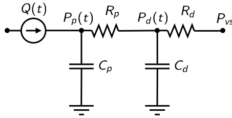
FIGURE 1 Visual representation of the two-stage Windkessel model of Eq. (1). In this electrical analogy, current represents blood flux, while voltage represents blood pressure. The heart is represented as a current generator, while the arterial network comprises dissipative and compliant elements, represented by resistances and capacitors, respectively.
