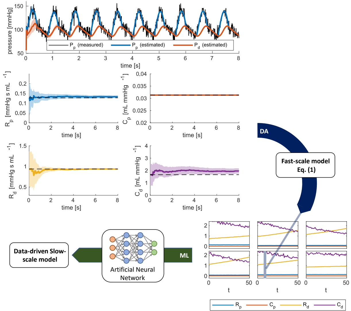
FIGURE 14 Test Case 4: visual representation of the procedure followed to generate a data-driven model for hypertension development (see Sec. 3.4.2). In the top part of the figure we represent in black the noisy measurement of P_p associated with a given patient i and a to given slow-time instant \tau_j . The colored line represent the time evolution of estimated values of the system state ( P_p and P_d ) and of the four parameters ( R_p , C_p , R_d and C_d ). The shadowed areas represent the \pm 3\sigma bands, where \sigma denotes the standard deviation of the estimate. By combining the estimated values of the parameters obtained for all patients and for all the slow-time instants, we obtain an estimate of their slow-scale evolution, represented in the bottom-right part of the figure.
