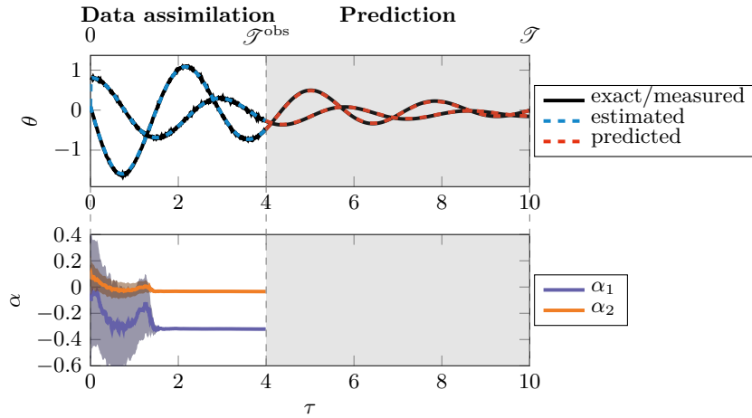
FIGURE 11 Test Case 3: evolution of \theta^{N_{P+1}}(\tau) , of \hat{\theta}^{N_{P+1}}(\tau) and of the estimation of \hat{\alpha}^{N_{P+1}} . See caption of Fig. 5 for the notation.
