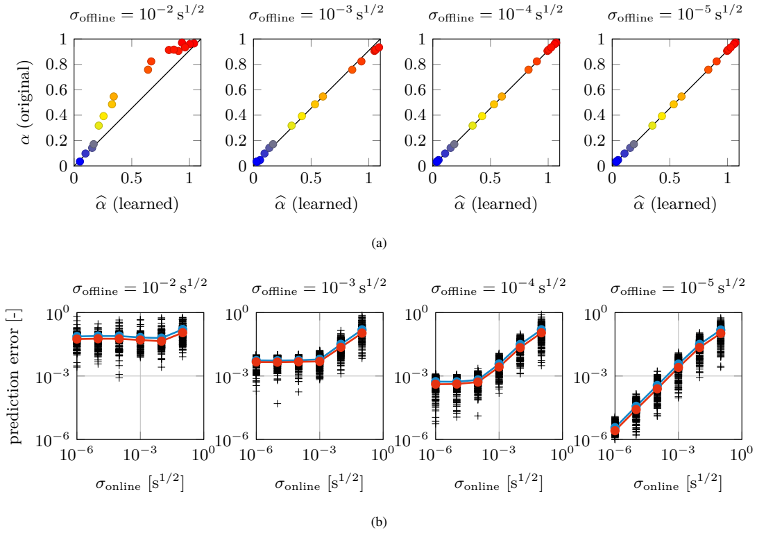
FIGURE 9 Test Case 1: (a) original parameters \alpha^i plotted against the corresponding learned parameters \hat{\alpha}^i for the training individuals ( i = 1, \dots, N_p ), for different noise magnitudes \sigma_{\text{offline}} and (b) overall L^2 relative prediction errors obtained for different values of \sigma_{\text{offline}} and \sigma_{\text{online}} . In (b), each black cross represent a testing individual, the blue curve represent the arithmetic mean, the red curve the geometric mean.
