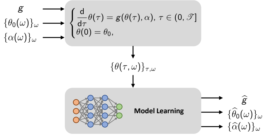
FIGURE 3 Visual representation of the idealized situation considered in Sec. 2.3.
