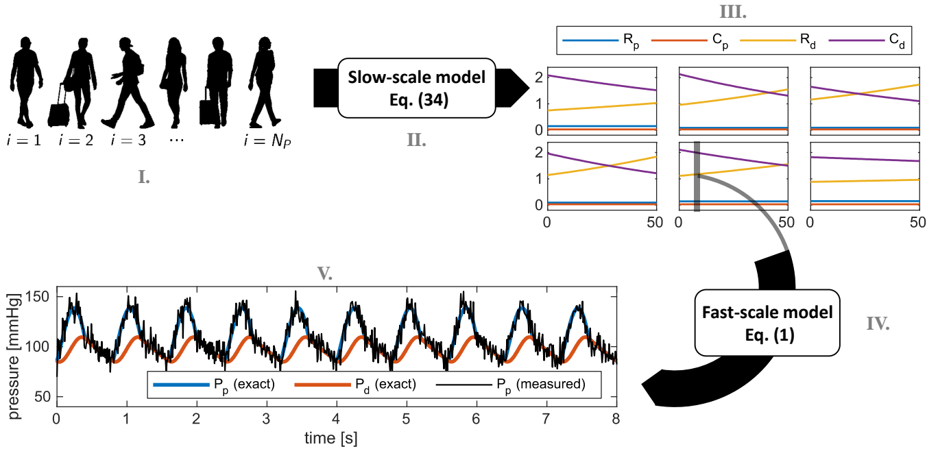
FIGURE 13 Test Case 4: visual representation of the five steps followed to generate synthetic data (see Sec. 3.4.1).
