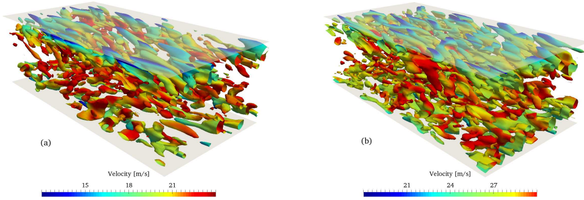
Fig. 10 Iso-surfaces of the Q-criterion ( Q = 50u_\tau^2/\delta^2 ) colored by the velocity magnitude, channel flows at (a) Re_\tau = 1000 and (b) Re_\tau = 20000 , HTLES calculation using grids B1 and D1, respectively.
