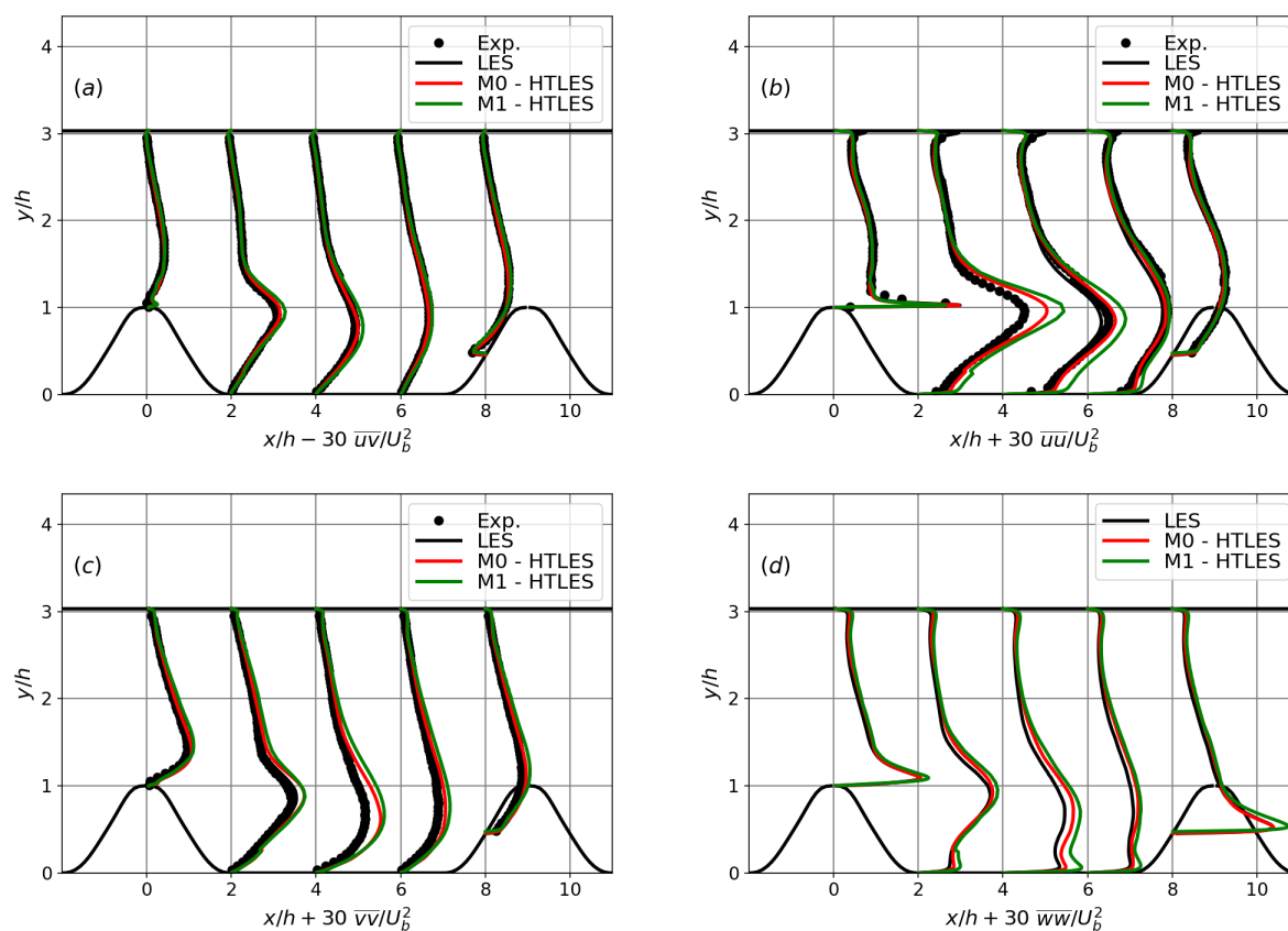
Fig. 25 Profiles of the modeled + resolved shear stress (a), streamwise (b), normal (c) and spanwise (d) components of the Reynolds stresses, periodic-hill flow at Re_b=10600 . HTLES results using grids M0 and M1.
