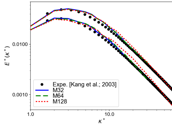
Fig. 4 Evolution of the resolved-energy spectra at two times. Reference data and k - \omega SST HTLES results on 3 grids (M32, M64, M128) with \beta_0 = 0.48 .
