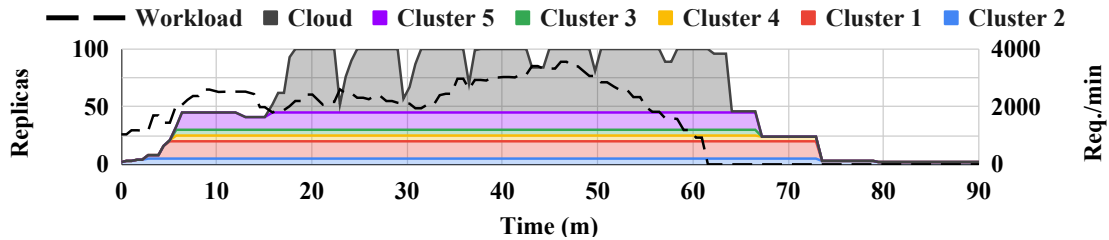
Fig. 9: No. replicas of the MCD during multi-cluster horizontal pod autoscaling and cloud bursting. Dashed lines represent requests per minute generated by the workload.
