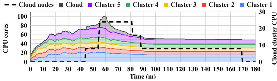
Fig. 6: Multi-cluster scheduling pods CPU request and cloud cluster lifecycle. Dashed line represents CPU cores of cloud nodes, whereas the stacked area represents the total CPU request of the pods running in the clusters.
