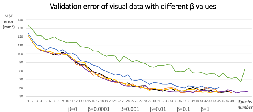
Figure 3: The impact of the gradual introduction of the regularization term (see equation 2) on the quality of the reconstruction of the visual data from the validation set.
