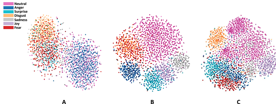
Figure 4: t-SNE plot [63] of the seven clusters of the latent representations formed by data distribution corresponding to the six emotions and the neutral state. The closest points in the higher dimensional space (latent variables size is 50) are the closest in the projection 2D space. The regularization term pushes data samples to gather around zero meanwhile maximizing their variance. The data samples were clustered differently depending on the nature of data (A: duration, B: acoustic and C: visual).
