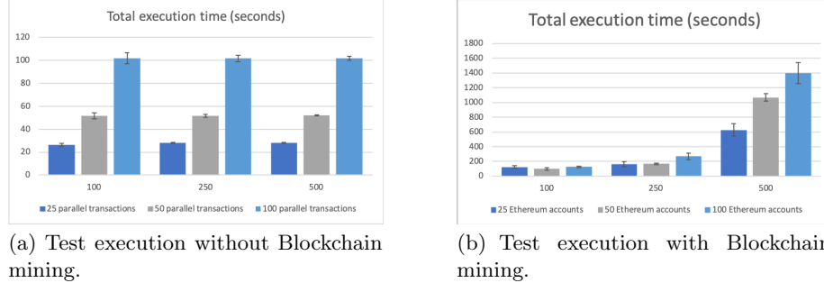
Fig. 3. Total execution time variation.
