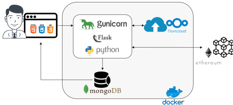
Fig. 2. SaaS software components.
