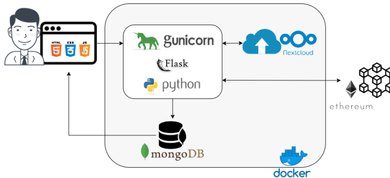
Fig. 2. SaaS software components.
