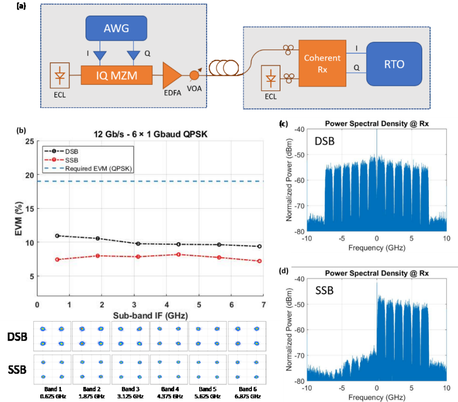
Fig. 1. (a) Experimental setup of the SSB generation using IQ modulation and coherent detection. (b) EVM Diagram per band and respective constellations for the DSB and SSB transmission in back-to-back configuration. (c) Recovered spectra after coherent reception of DSB and (d) SSB generated multiband schemes.
