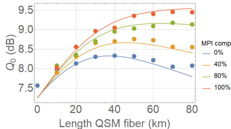
Fig. 3: Optimum Q-factor Q_0 as a function of the QSM fiber length \ell_{s_1} per span. (Symbols: Points: Monte Carlo simulations; Lines: Least squares fitting using (1)-(4) with \epsilon as an unknown parameter. Here \epsilon \simeq 0.2 .)
