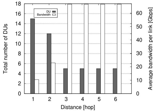
Fig. 9. Comparison of the average bandwidth per link and total active DUs as a function of the distance constraints for xhaul with the limitation on both processing units and hops in the high traffic (12 p.m.).
