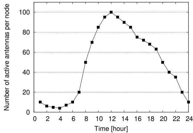
Fig. 4. Evolution of the number of active antennas per node during the 24 hours.
