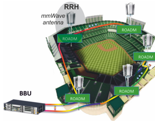
Fig. 1. Conceptual representation of the 5G IFoF/mmWave fronthaul architecture for hot-spot stadiums.
