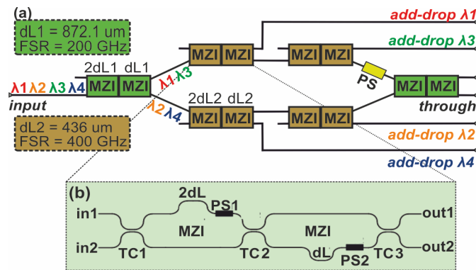
Fig. 3. a) ROADM design based on cascaded MZIs, b) building block of the cascaded MZIs.
