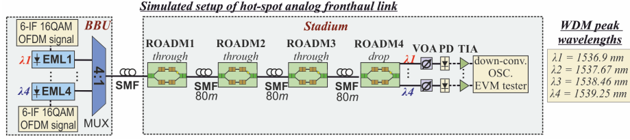
Fig. 5. Simulated setup of the analog multi - IFoF optical fronthaul, comprising the WDM EML-based transmitter at the BBU side and the ROADM bus at the stadium side.
