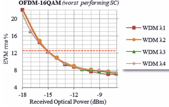
Fig. 7. EVM versus ROP (dBm) for the worst performing SC of each WDM channel.
