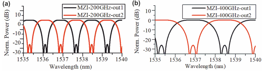
Fig. 4. ROADM modeling: Simulated spectral response of the cascaded MZIs' filters with: a) FSR = 200 GHz (green MZIs), b) FSR = 400 GHz (brown MZIs).
