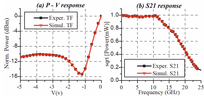
Fig. 2. EML modeling: a) Power versus Volts experimental and simulated transfer functions, b) experimental and simulated S21 curves.
