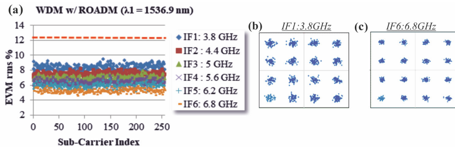
Fig. 6. a) EVM per sub-carrier for all IF bands for \lambda_1 = 1536.9 nm at a minimum received optical power of -13 dBm, b) constellation diagram for the first IF band at 3.8 GHz and c) the last IF band at 6.8 GHz.
