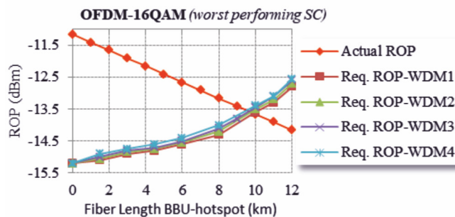
Fig. 8. ROP versus the length of the SMF fiber connecting the BBU with the first ROADM. Curve of the actual ROP deriving from the power budget of the hot-spot link and curves of the ROP required to achieve an EVM = 12.5 % (3GPP threshold) for all WDM channels.
