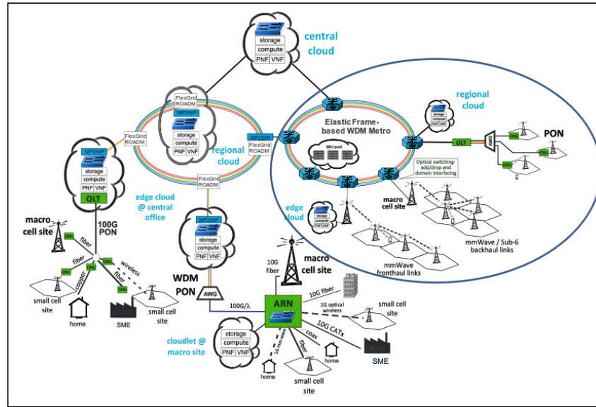
Fig. 1. Physical architecture - converged fixed-mobile 5G network
