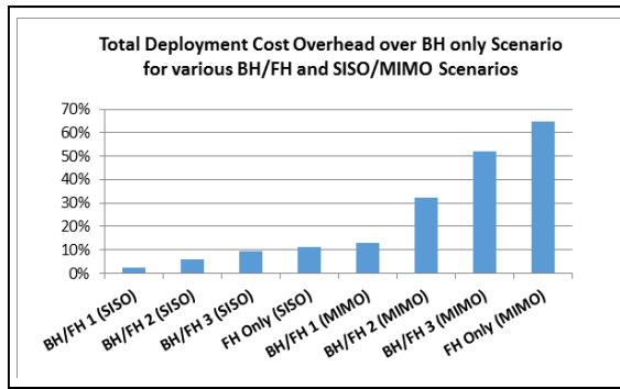
Fig. 6. Comparative Cost for various BH/FH and SISO/MIMO Transport Network Deployment Scenarios
