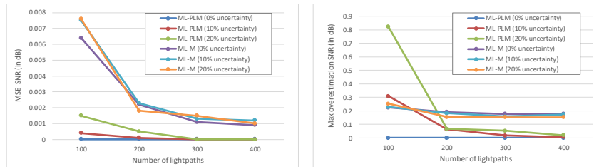
Fig. 3 a) MSE and b) maximum overestimation for 0%, 10% and 20% uncertainty.
