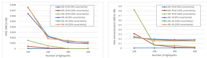
Fig. 3 a) MSE and b) maximum overestimation for 0%, 10% and 20% uncertainty.
