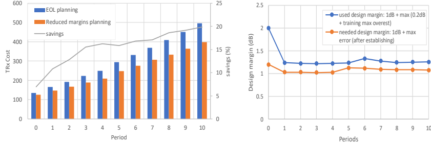
Fig. 4: a) Total cost (in cost units) and savings of elastic transponders (ET) per period when planning with accurate QoT estimation/reduced margins and with high margins, b) Used and needed design margin.
