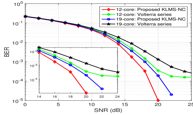
Fig. 6. SNR vs BER performance for the proposed KLMS algorithm for 12-core and 19-core MCF using 16-QAM
