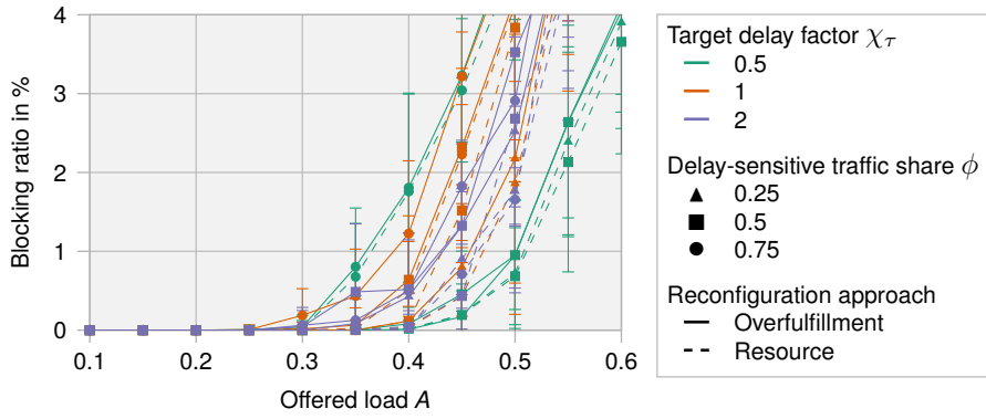
(c) Blocking ratio.
