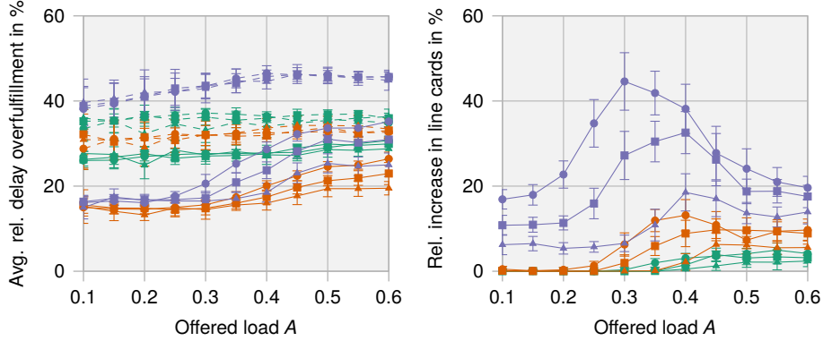
(a) Average relative delay overfullfillment. (b) Relative increase in required line cards.
