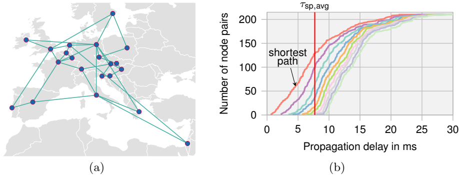
Fig. 3. Logical fiber topology (a) and propagation delay distributions of the 10 shortest paths (b) for the European research network Géant [9] without the node in New York. The path length index in (b) increases from left to right, i.e., the red curve on the left corresponds to the shortest path. The average delay of the shortest path at \tau_{sp,avg} = 7.7 ms is depicted with the red vertical line.
