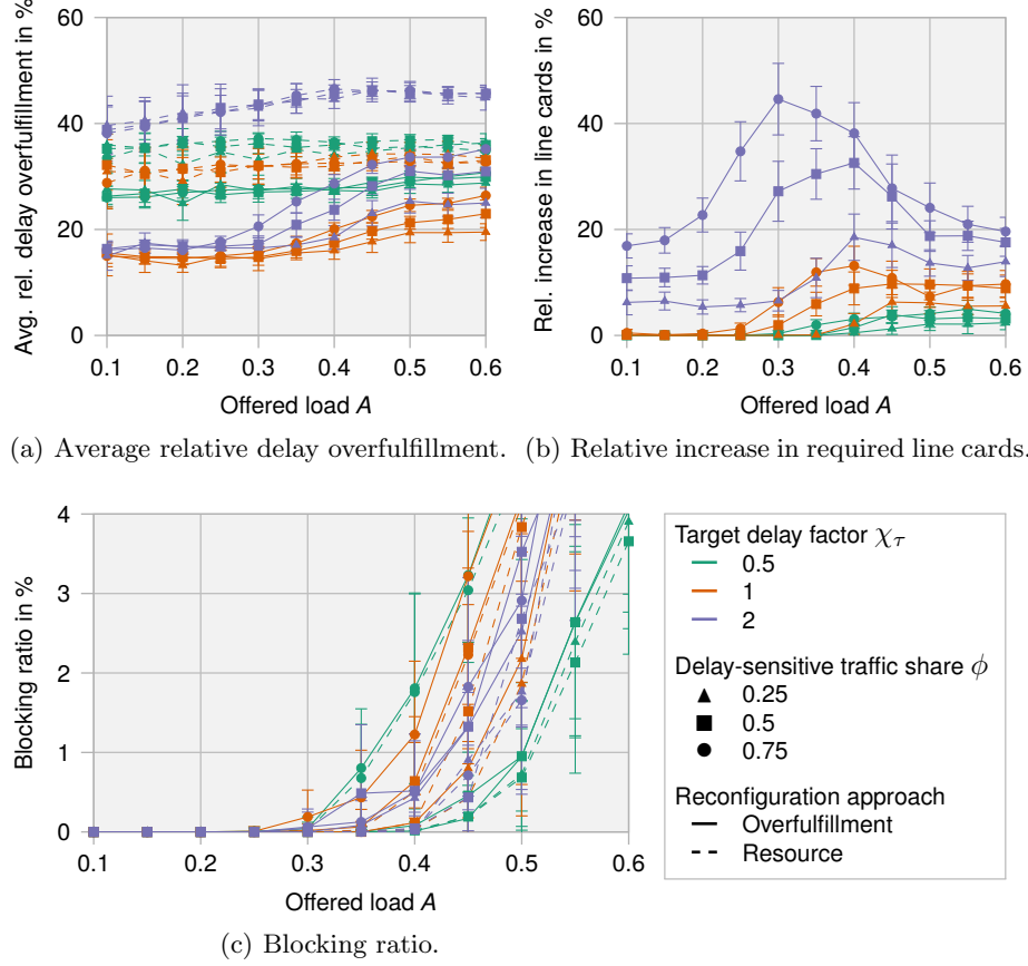
Fig. 4. Results of the introduced reconfiguration approach for wavelength demands with Poisson arrivals and departures. Shown metrics are the average relative delay overfullment (a), the relative increase in required line cards compared to a delay-aware resource optimization (b) and the blocking ratio (c). The error bars represent one standard deviation.
