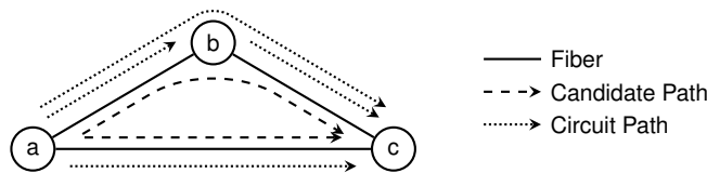
Fig. 2. Candidate path generation for a demand from node a to node c.
