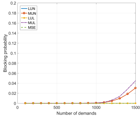
Fig. 5. Blocking probability using different sorting techniques.
