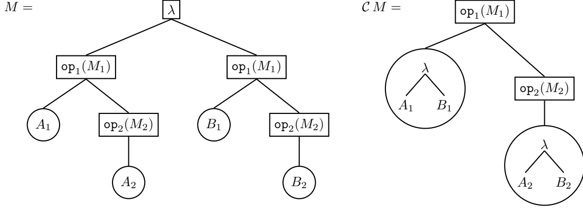
Figure 3: Example of applying the \mathcal{C} operator to a term.
