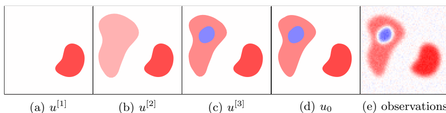
Fig. 1: First experiment ( u^{[k]} is the k -th iterate produced by Algorithm 1)
