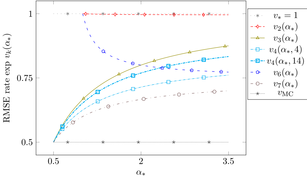
Figure 4: Plots of the negative exponent v_k(\alpha_*) of the optimal rate at which the estimator RMSE decreases as functions of \alpha_* . Functions v_2(\alpha_*) and v_6(\alpha_*) require V_{\text{HK}}(h) < \infty , so they are shown for only \alpha_* \geq 1 because of (14).
