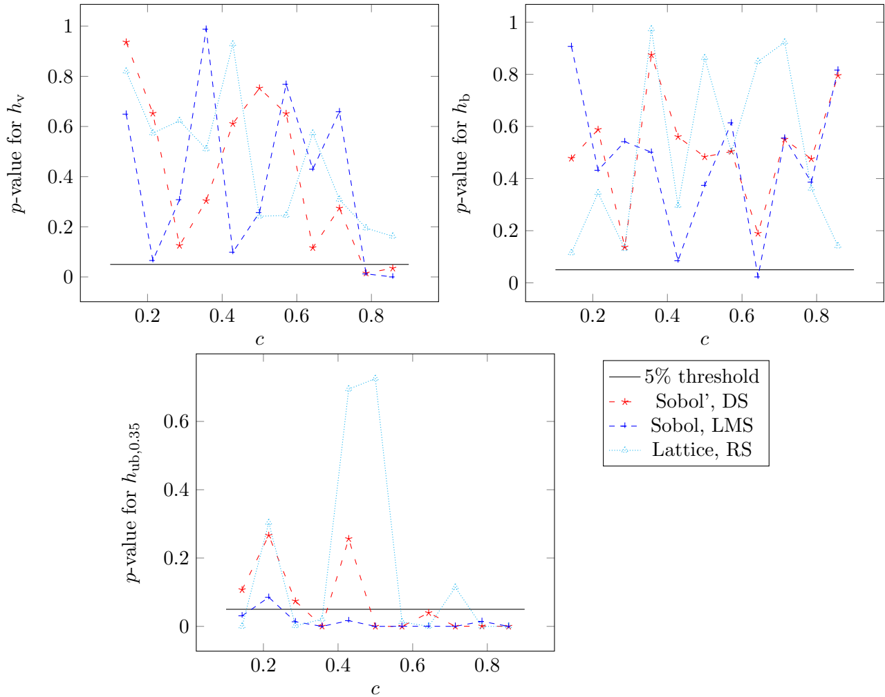
Figure 5: p -values of the Shapiro-Wilk test for various values of c = t/14 for 2 \leq t \leq 12 and for three RQMC techniques with n = 2^{14} , from 100 independent estimations. The considered integrand is h_v (top left), h_b (top right) and h_{ub,0.35} (bottom left), each for dimension s = 4 .
