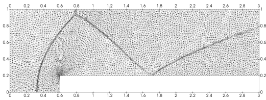
(b) Adapted h = 0.0025 mesh at t = 2.0 .
