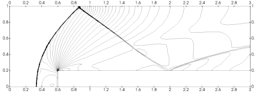
(c) Adapted h = 0.0025 mesh at t = 1.5 .
