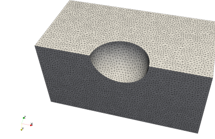
(b) Shock-sphere test case.
