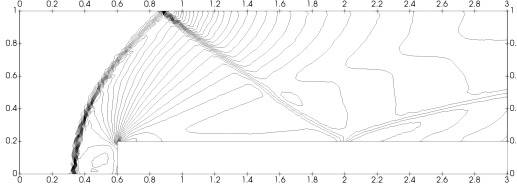
(a) Nonadapted h = 0.0025 mesh at t = 1.5 .
