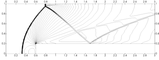
(e) Fine (nonadapted) h = 0.00125 mesh at t = 1.5 .
