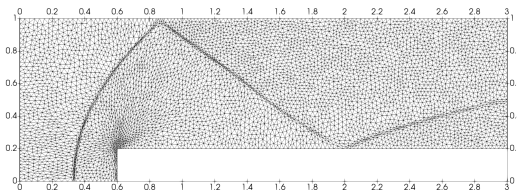
(a) Adapted h = 0.0025 mesh at t = 1.5 .
