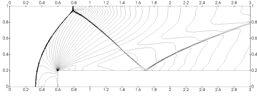
(d) Adapted h = 0.0025 mesh at t = 2.0 .
