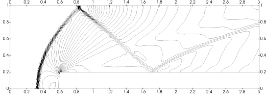
(b) Nonadapted h = 0.0025 mesh at t = 2.0 .
