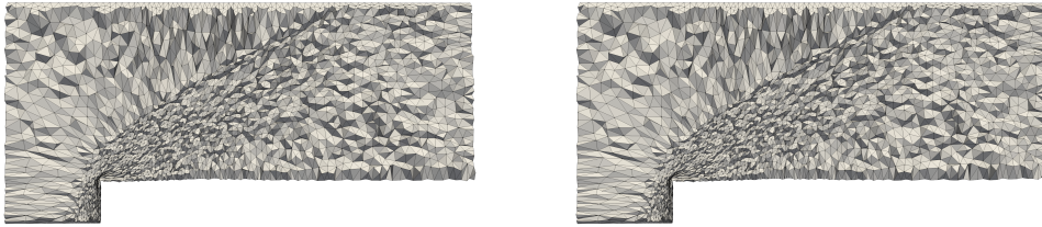
Figure 16: Three-dimensional forward facing step adapted meshes at t = 1.5 and t = 2.0 .
