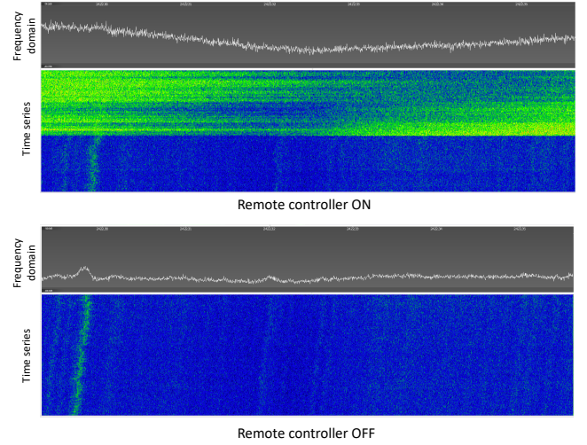
Fig. 3: Spectral analysis of the impact of turning on the UAV RC for a common commercial device (FrSky Taranis X9D 2.4G ACCST). Center frequency: 2422.26 MHz.
