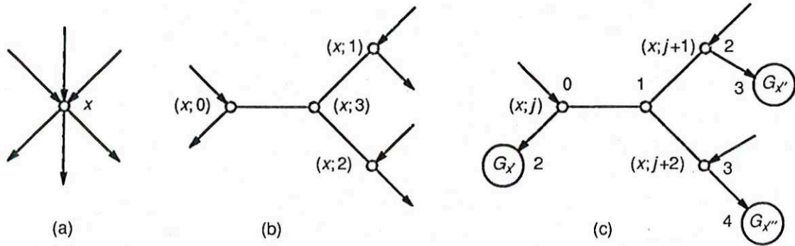
FIG. 4.2. Replacing a vertex with a 3-star.
