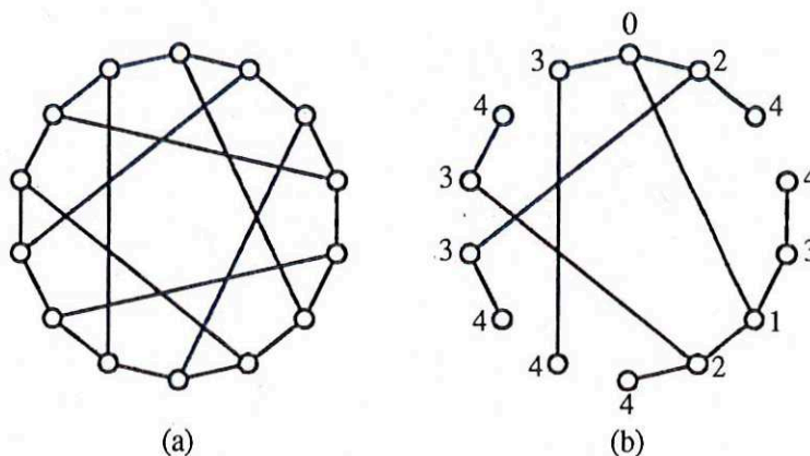
FIG. 7.1. Heawood graph (a) and its broadcast scheme (b).
