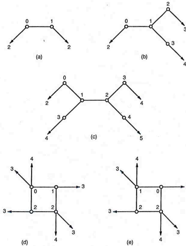
FIG. 6.1. Average time.
