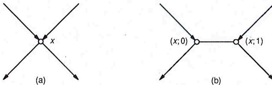
FIG. 4.1. Replacing a vertex with an edge.
