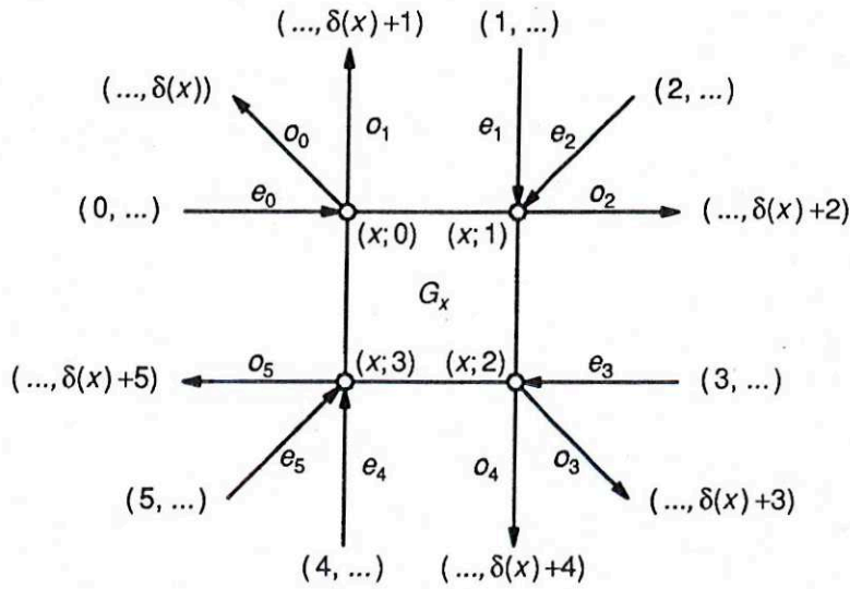
FIG. 5.1. Replacing a vertex with a C_4 .
