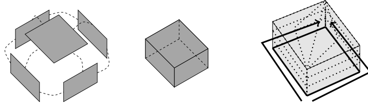
Figure 3: Fahrenberg's matchbox M and two non-dihomotopic dipaths
