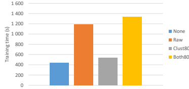
Fig. 3: Average training time over all the datasets
