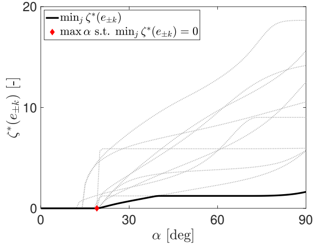
Fig. 6. Grey lines show the resulting displacement \zeta^* toward all positive and negative base vectors, i.e., e_{\pm k} = \pm \partial / \partial I_k , k = 1, \dots, n . Black line shows the minimum of these curves. The minimal angle \alpha ensuring local controllability is highlighted in red. One can notice that some curves do not strictly increase, but are constant instead. It means that the control is inside the cone, and increasing \alpha does not change the result.
