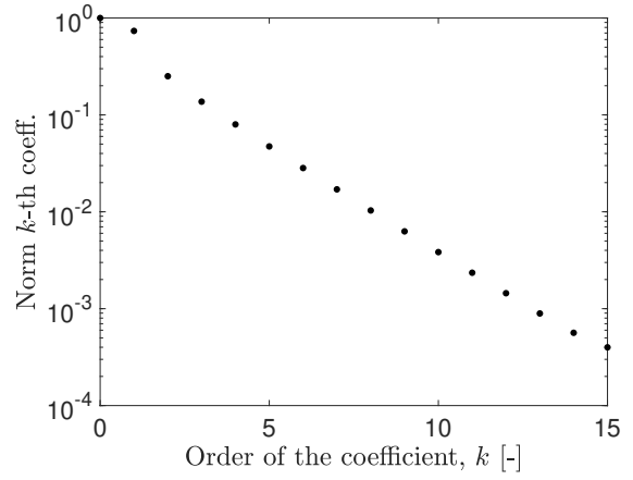
Fig. 5. Convergence of coefficients of the DFT. The norm is evaluated as \sqrt{\sum_i |\int_{\mathbb{S}^1} F_i e^{ik\varphi} d\varphi|^2} / \sqrt{\sum_i |\int_{\mathbb{S}^1} F_i d\varphi|^2} .
