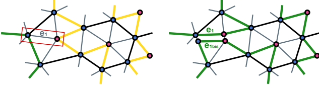
Figure 8: Connecting cycles through edge doubling. Left: an unused edge e_1 (in red quad) between two different cycles (in green and yellow). Right: the two cycles are joined together after doubling the edge e_1 and its endpoints, adding an extra edge e_{1bis} .
