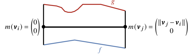
Figure 28: The segment cell boundary is represented by two functions f, g .
