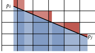
Fig. 25. The vector field's integral under a segment is obtained by decomposing it in smaller segments contained in single quads of the grid.
