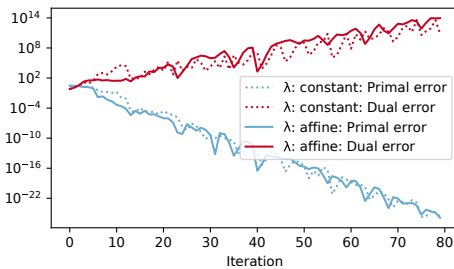
Fig. 4: Convergence rate: every iteration, \lambda is updated and \mu is increased by a factor of 3
