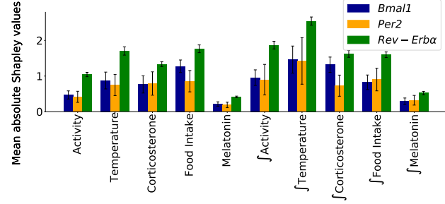
Fig. 4. Mean absolute Shapley values for all features and each gene under (H1-H3). Standard deviations computed across residual trajectories.
