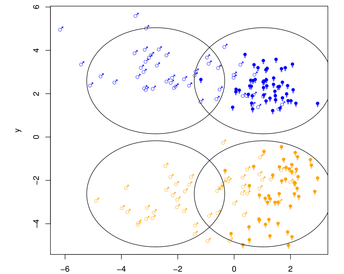
Figure 3: Crab dataset on the two clustering components
